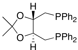
DIOP
