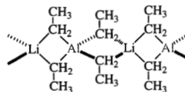
(11) [\text{LiAl}(\text{C}_2\text{H}_5)_4]_n
